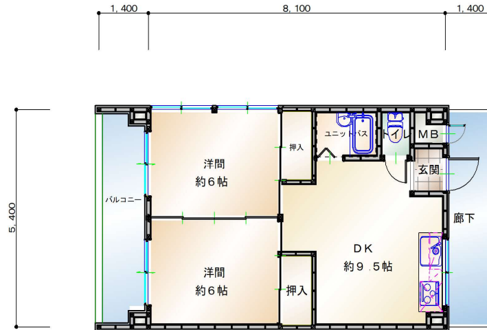
間取
